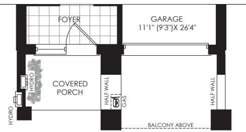
PARTIAL GROUND FLOOR PLAN ELEV. 'F'
