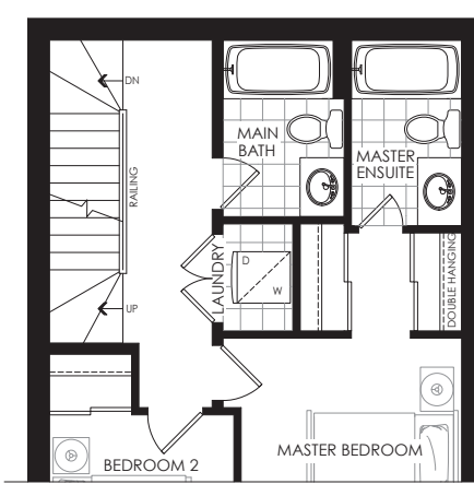
PARTIAL THIRD FLOOR FLEX PLAN WITH LAUNDRY ELEV. 'A','B' WITH ROOF TOP TERRACE
