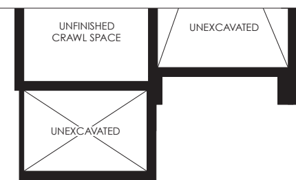
PARTIAL CRAWL SPACE PLAN ELEV. 'C'
