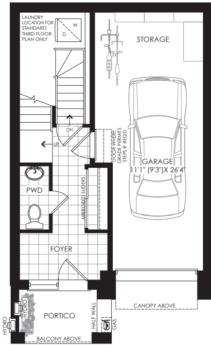
GROUND FLOOR PLAN ELEV. 'A','B'
